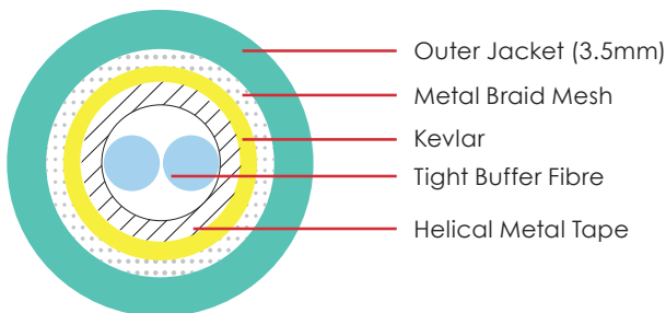
Duplex OM3 Fibre Patch Lead Diagram
