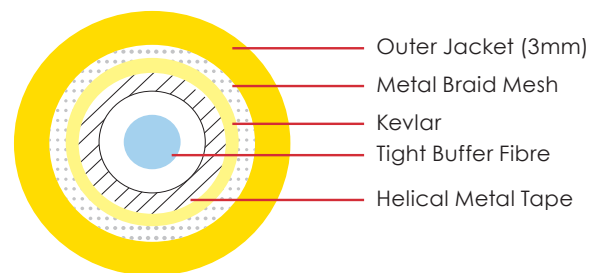
Simplex OS2 Fibre Patch Lead Diagram
